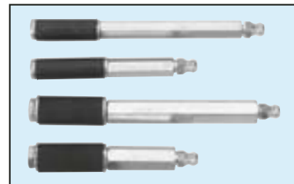
Standard crack injector steel or aluminium available in sizes from D 10/70 to D 20/200
